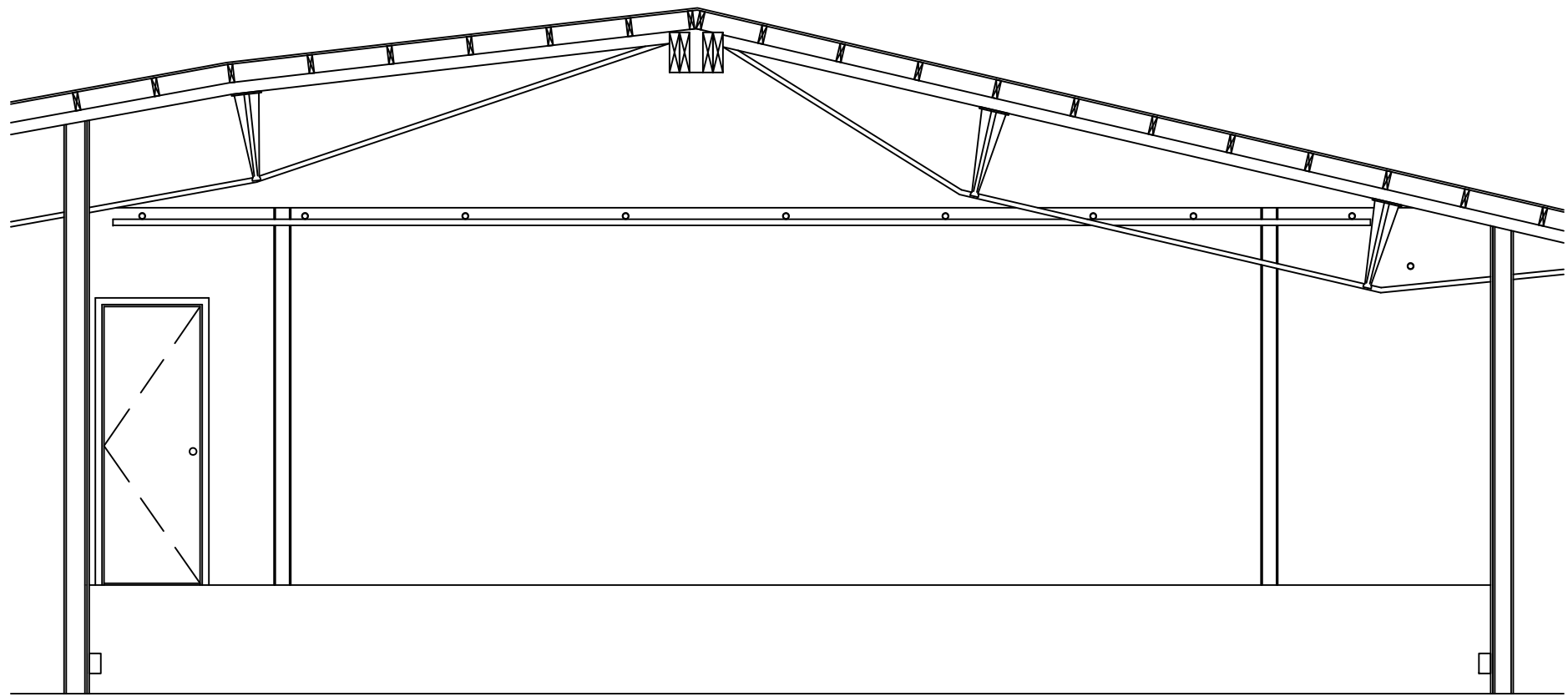
2 Transverse Section
