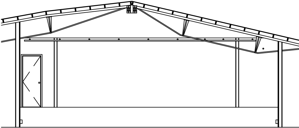
Transverse Section
